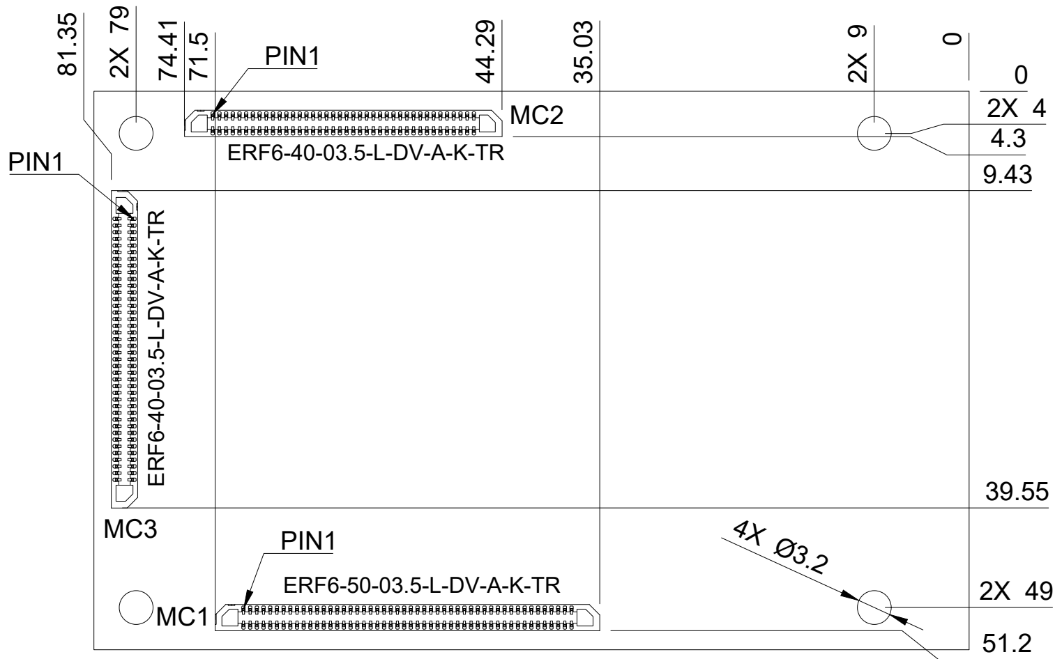
Top View
