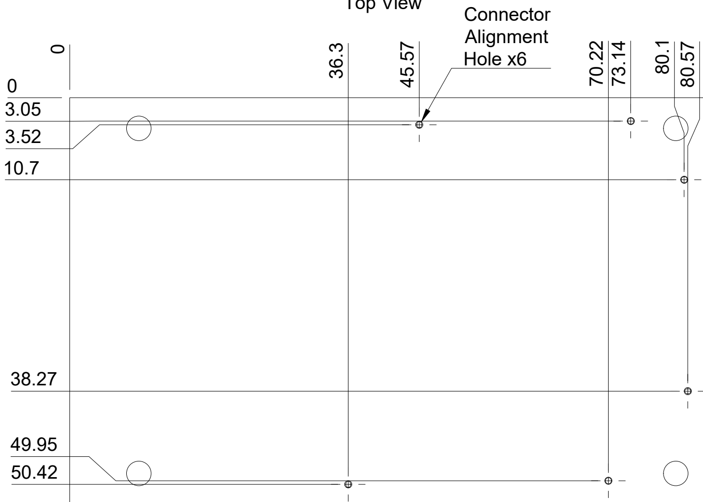
Bottom View
